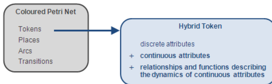
Figure 1. Components of coloured stochastic Petri net with hybrid tokens
