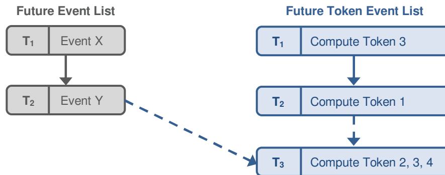
Figure 3. Structure of future event list and future token event list and connection between them
